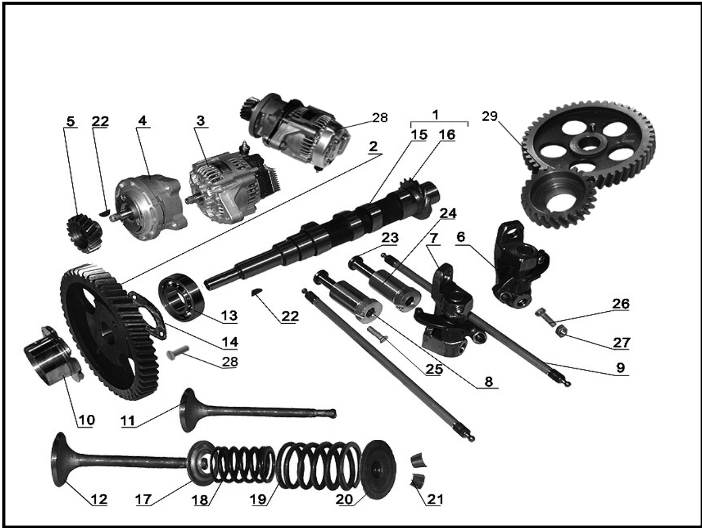
Figure 6. - Timing Gear
