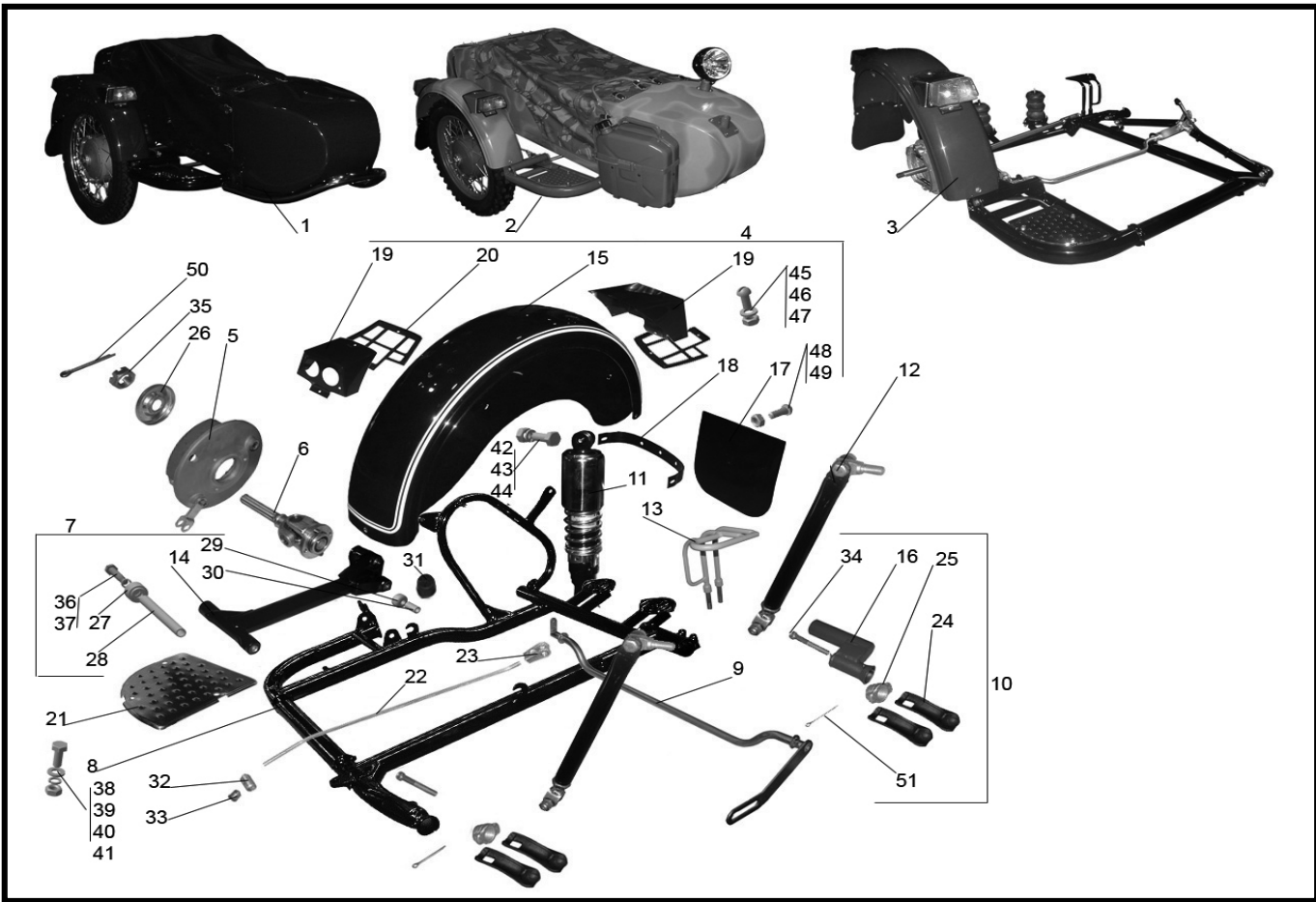
Figure 35. - Sidecar Frame, 2WD
