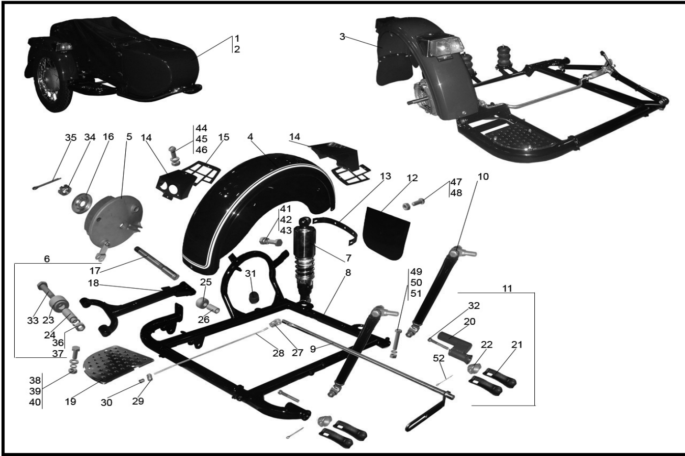
Figure 34. - Sidecar Frame, 1WD
