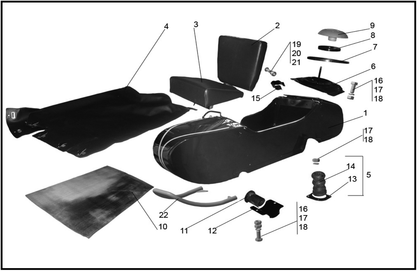
Figure 36. - Sidecar Body, Standard
