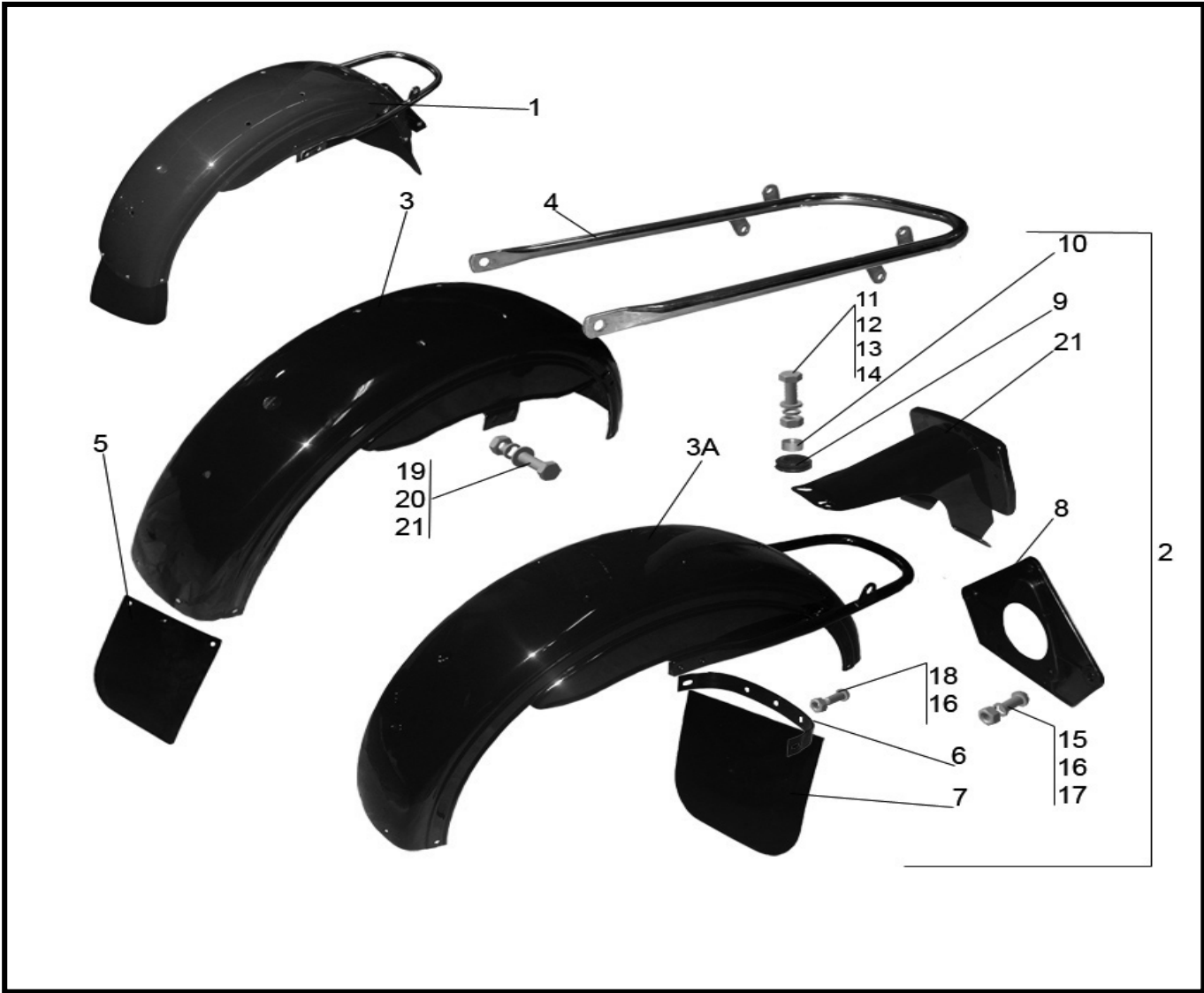
Figure 23. - Rear Fender
