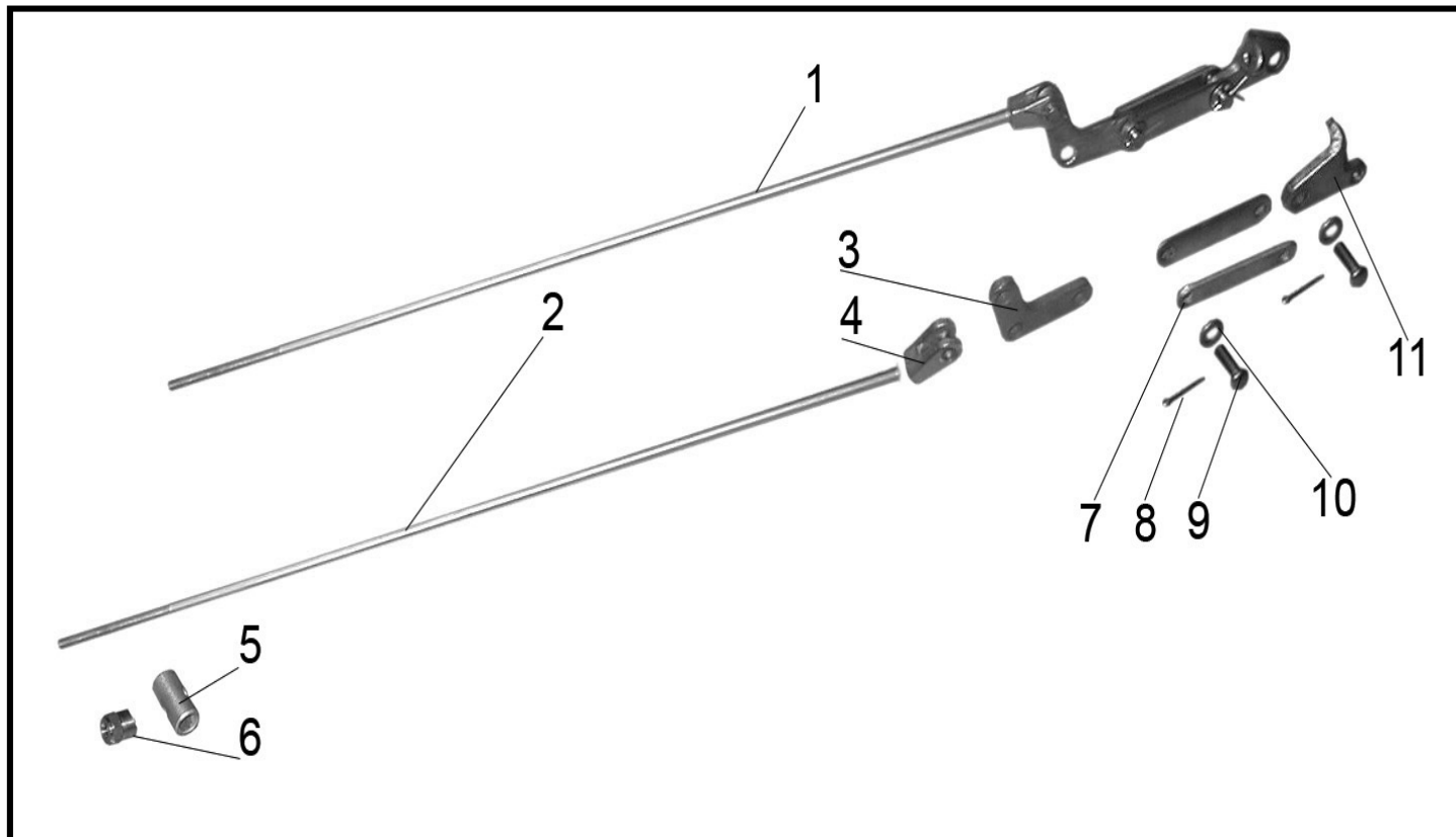
Figure 26. - Rear Brake Linkage
