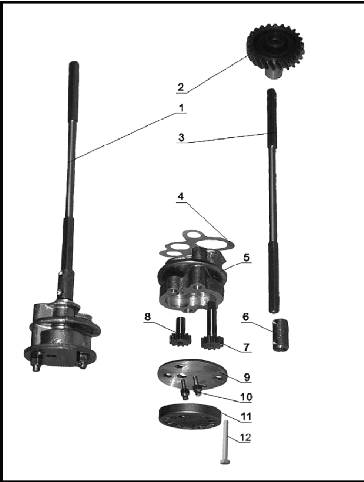
Figure 7. - Oil Pump
