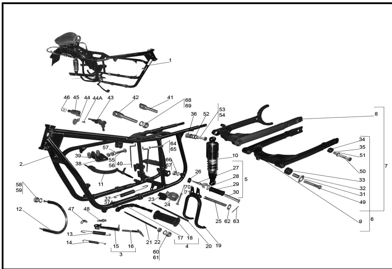
Figure 22. - Motorcycle Frame
