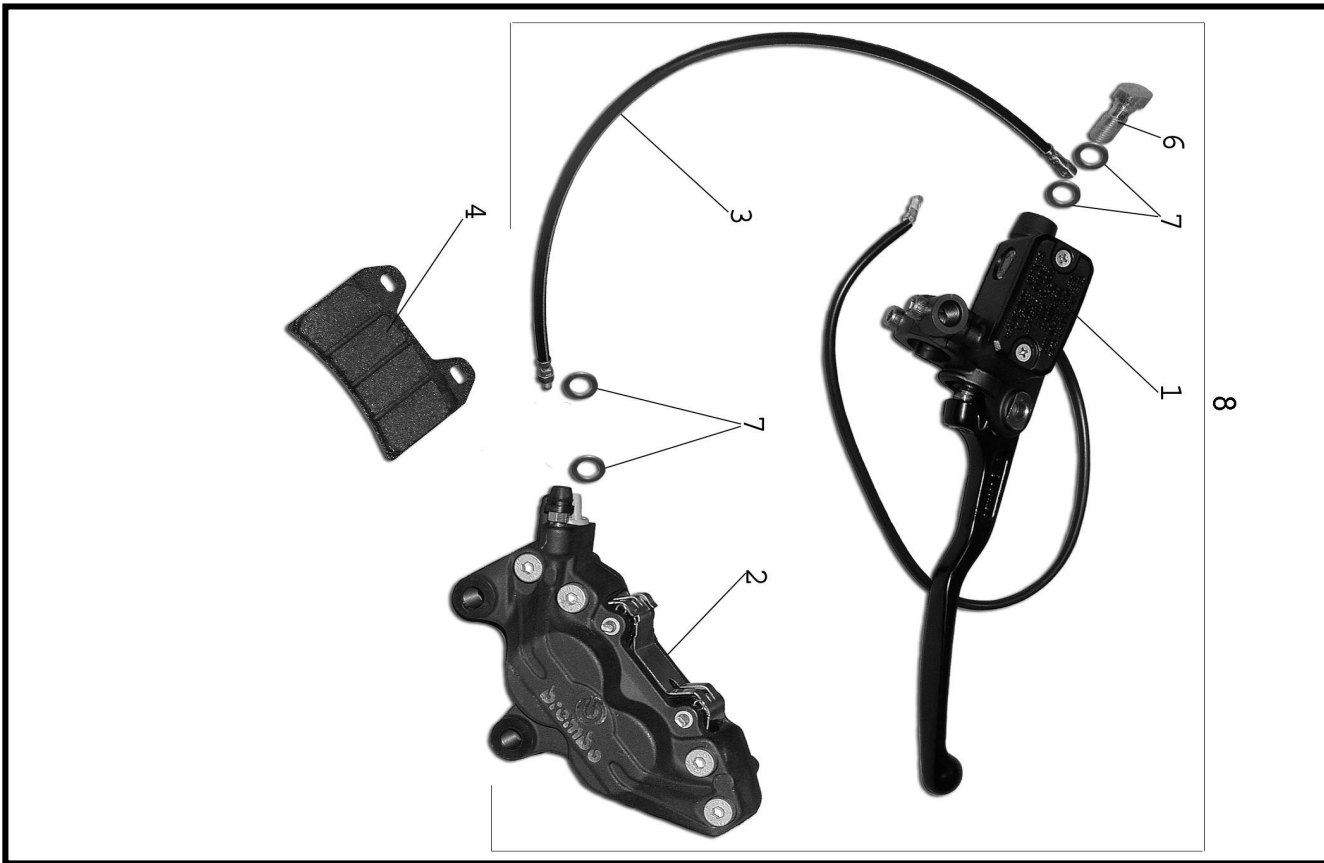
Figure 40. - Hydraulic Brake
