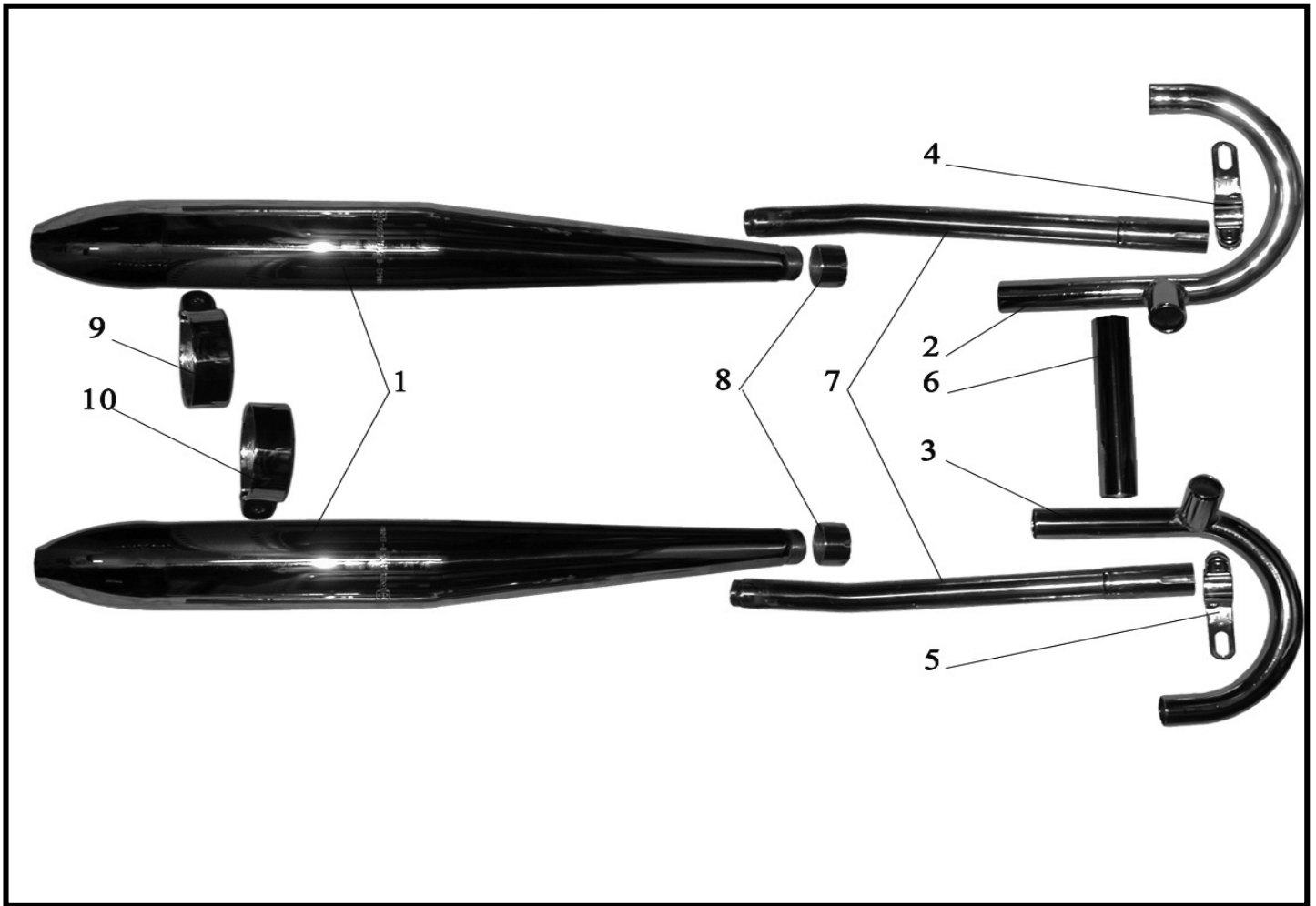
Figure 27. - Header Pipes, Mufflers
