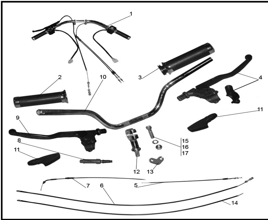
Figure 25. - Handlebar and Controls
