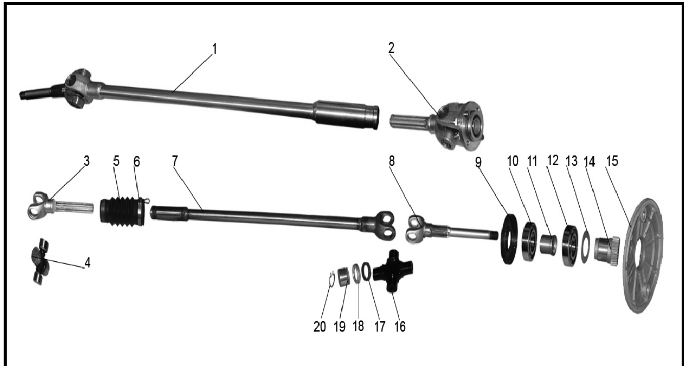
Figure 15. - 2WD Shaft
