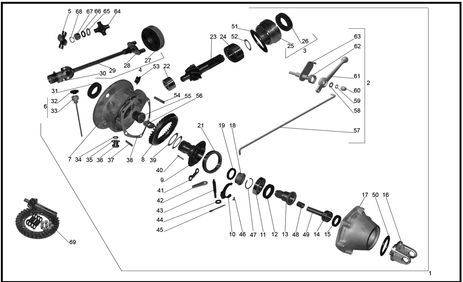
Figure 14. - Final Drive 2WD
