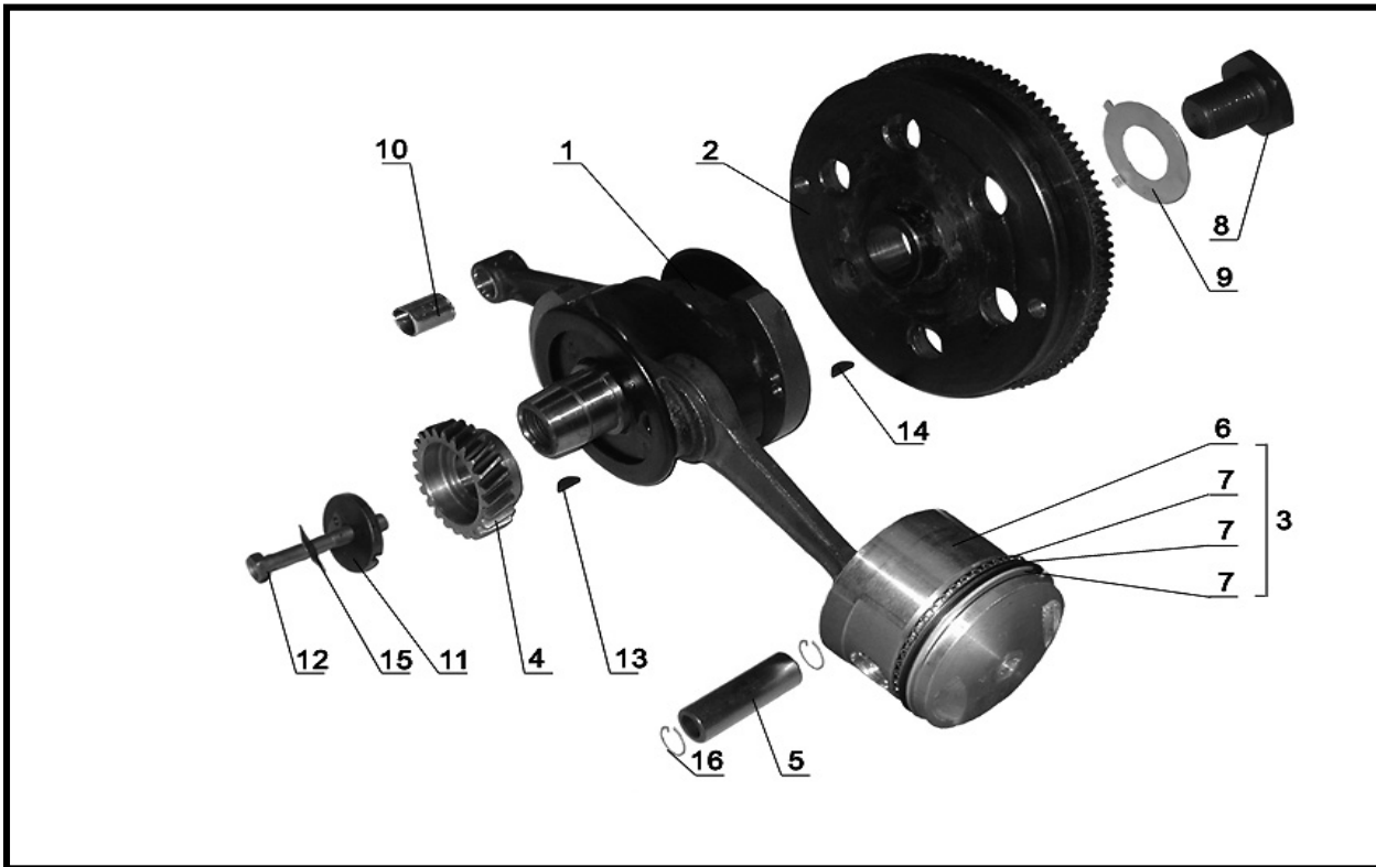
Figure 4 - Crankshaft with Rods and Pistons
